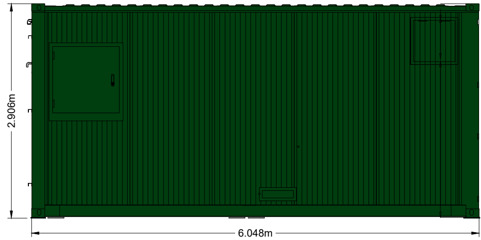
EASTERN ELEVATION
