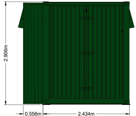
NORTHERN ELEVATION
