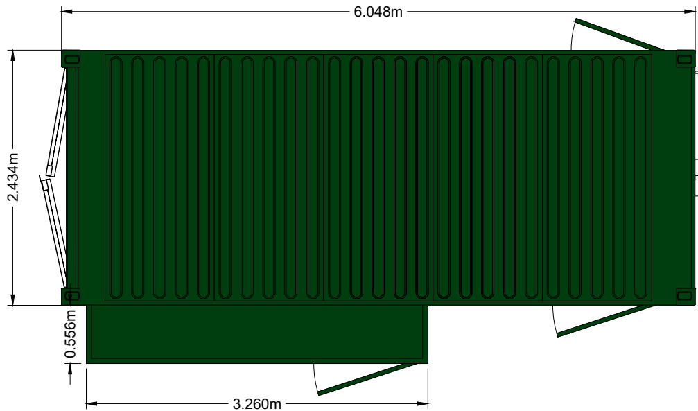
ROOF PLAN
