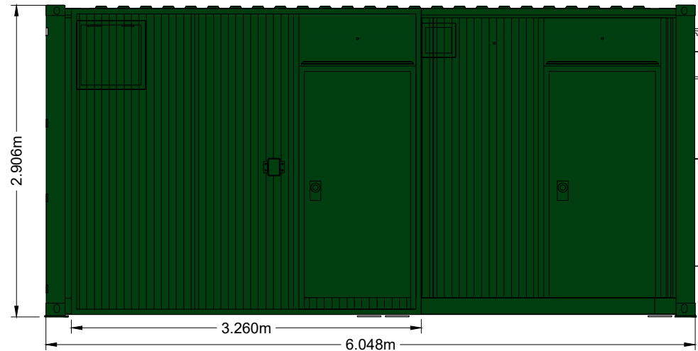
WESTERN ELEVATION
