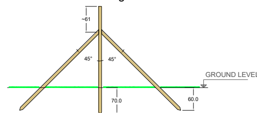
Middle Shoring Post
