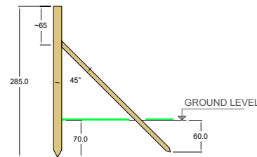
Initial Shoring Post
